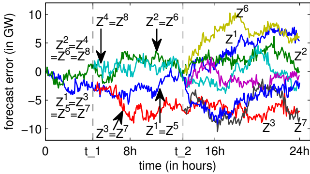
Figure 2: Example of possible trajectories of the forecast errors. To ease the presentation, this example has only eight trajectories. The numerical results of Section 6 use 512 trajectories. These trajectories are generated using data from the UK (see §6.1).
