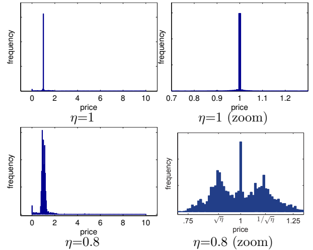
Figure 7: Distribution of prices for a system equipped with storage of capacity C_{\text{max}} = 5\text{GW} , B_{\text{max}} = 5\text{GWh} and charge-discharge efficiency \eta = 1 or 0.8 . For readability, we scale the values c, v and c^{bo} to c = 1 .
