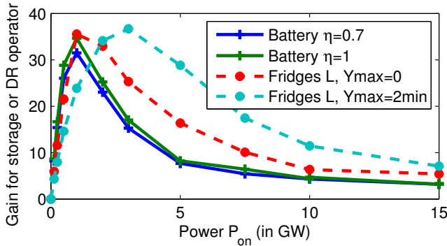
Figure 9: Revenue for the DR or storage operator as a function of the installed capacity. The studied scenarios are the same as in Figure 6.
