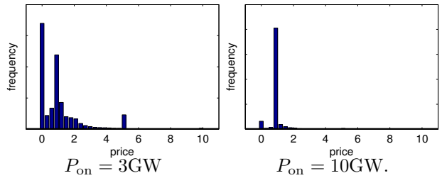
Figure 8: Distribution of prices for a system equipped with DR appliances Fridges L with Y_{\text{max}} = 20\text{min} . For readability, we scale the values c, v and c^{bo} to c = 1 .
