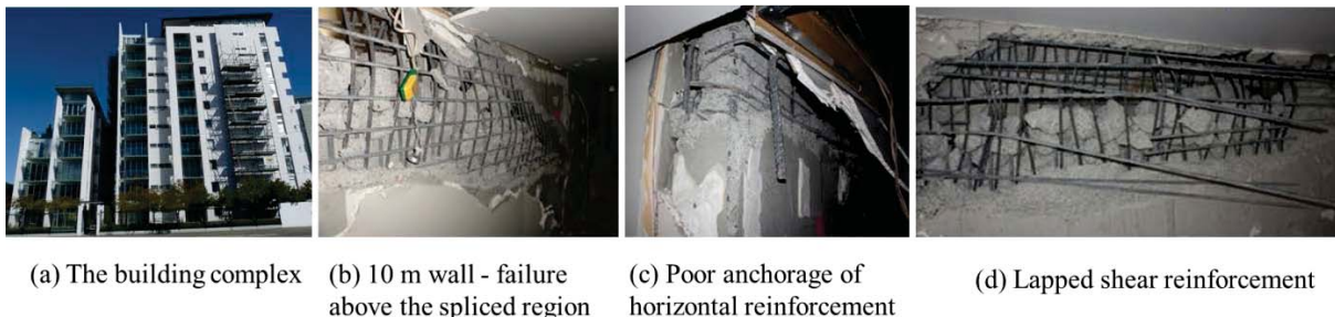
Figure 10 Performance of a concrete wall in one building of the Terrace on the Park
