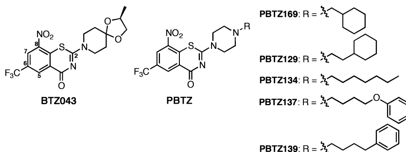
Figure 1. Chemical structures. Structure of BTZ043 and five compounds of the PBTZ family selected for in vivo studies, PBTZ169, PBTZ139, PBTZ134, PBTZ137 and PBTZ129.
