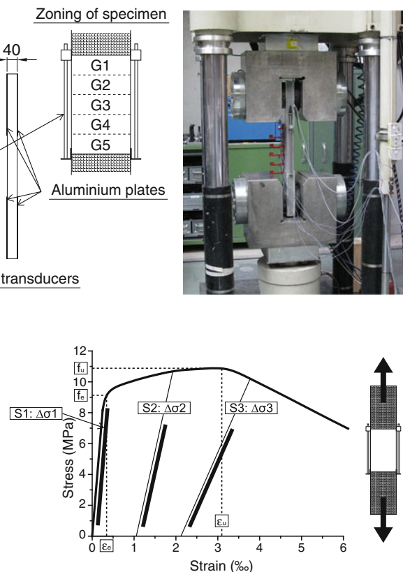
Fig. 4 Schematic representation of tensile response of UHPFRC and definition of tensile fatigue test series
