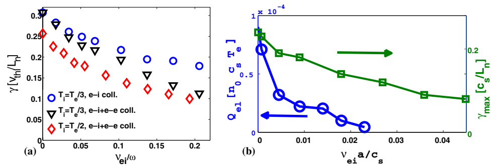
Figure 8. (a) Collisional damping of linear growth rates in the TEM regime. The TEM TCV case with a/L_{Ti} = 0 , a/L_{Te} = 1.70 , a/L_n = 0.85 , mode k_\theta \rho_{Li} = 0.4 . The electron-ion collision frequency \nu_{ei} is normalized with respect to \omega , the collisionless real frequency of the considered mode k_\theta \rho_{Li} = 0.4 . (b) The small TEM CYCLONE case, T_i = T_e/3 . Electron collisionality scan, both for the quasi-stationary electron turbulent energy flux Q_{ei} , averaged between r/a = 0.4 and r/a = 0.6 , and for the maximum linear growth rate \gamma_{\max} . Electron collisions have a damping effect on TEM instabilities both in linear and non-linear simulations, the damping of non-linear turbulent transport (compared with a collisionless case) being however stronger than the damping of linear growth rates.
