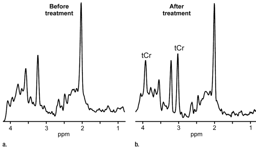
Figure 5: 1 H MR spectroscopy of neurometabolic disorder. (a, b) White matter spectra (1.5 T, PRESS MR spectroscopic imaging, 3000/30, six weighted averages, nominal voxel size = 10 × 10 × 15 mm 3 ) in girl with guanidinoacetate methyltransferase deficiency before treatment at age 3 years 2 months (a) and after 3.5 months of treatment with oral creatine supplementation (b). Resonance from creatine-containing metabolites (tCr) returned to normal in this region as well as in other investigated brain areas.
