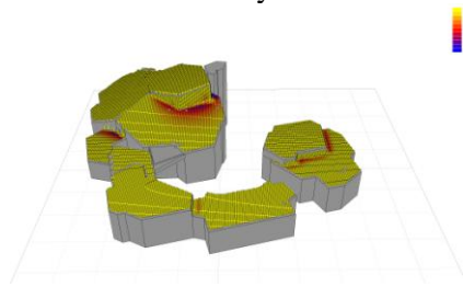
Fig.2 Annual Solar Radiation Analysis via Ecotect
