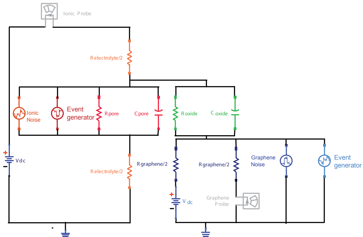
SI Figure 7. Schematics of the simplified lumped element model of our device used to analyse and test if the signal transmitted in the part of the circuit related to ionic current detection creates an undesired effect in the graphene circuit and vice versa.
