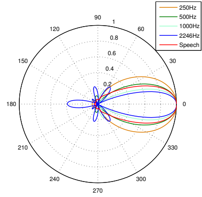
Fig. 4. Speech beam-pattern vs. narrowband beam-pattern for superdirective beamformer with circular microphone array.
