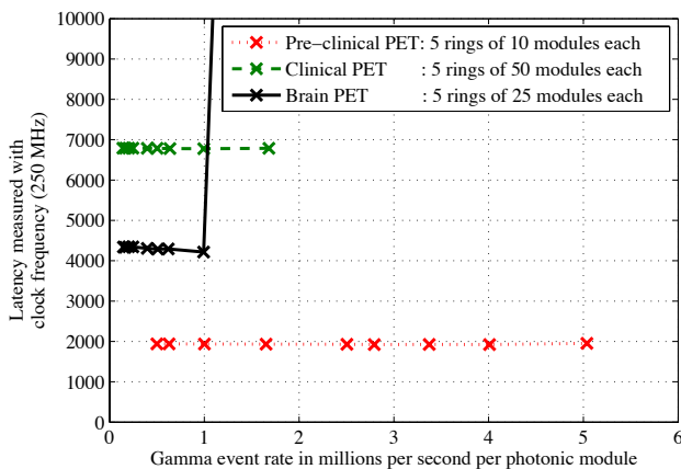
Figure 13. Network latency as a function of Gamma event rate for pre-clinical, brain, and clinical PET configurations.
