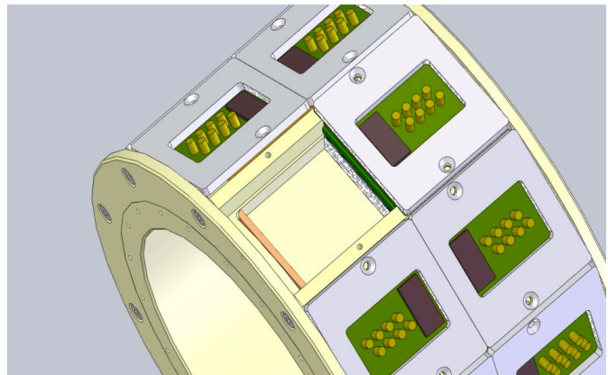
Figure 15. CAD drawing of the final MRI compatible pre-clinical system assembly.
