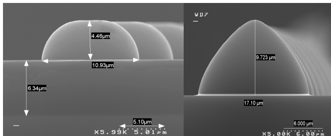
Figure 4. Concentrators fabricated at the interface between scintillator and sensor tile.
