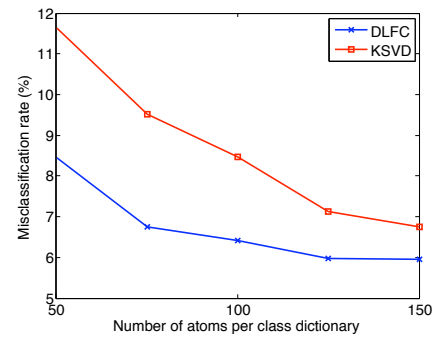
Fig. 4. Variation of the classification error with dictionary size.
