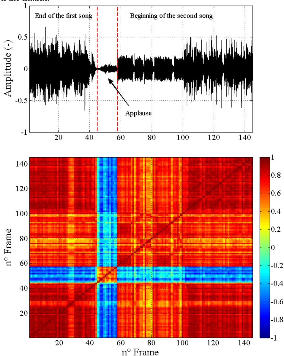
Figure 1: top: waveform of a song change, bottom: corresponding similarity matrix.
