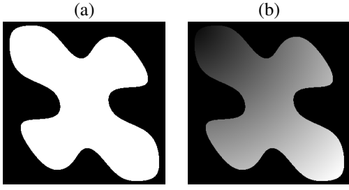
Fig. 1. A continuous domain edge image, which is discontinuous on some predefined curve. The discontinuity across the curve can be (a) uniform or (b) varying in general.
