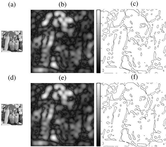
Fig. 14. Reconstruction of FRI curve model for natural images from (a) ideal and (d) Bicubic low-pass filtered samples of the high-resolution ground truth image. (b) and (e) Reconstructed mask function. (c) and (f) Roots of the mask function, i.e. the annihilable curve. The order of the FRI model is 29 \times 29 .
