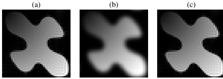
Fig. 6. (a) Samples with ideal sinc kernel. (b) Samples with Gaussian kernel. (c) Samples obtained by applying additional post-filtering. The SNR of (b) and (c) compared with the ground truth (a) are 13.47 dB and 38.39 dB respectively.
