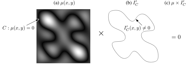
Fig. 2. Spatial domain interpretation of the annihilation equation (4). The function \mu(x, y) , whose roots defines the curve, serves as a mask to annihilate whatever is different from zero in the derivative image I'_C (see text in Section II-C2).
