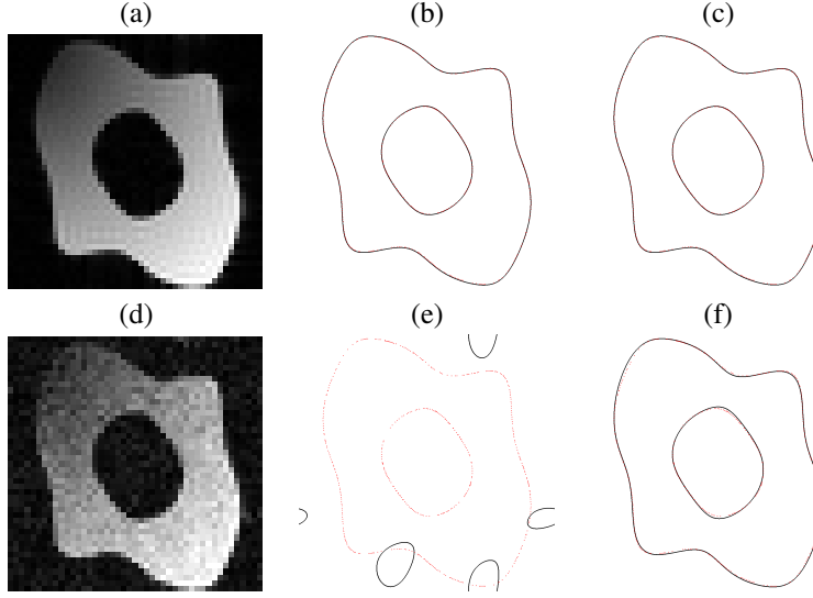
Fig. 10. Reconstruction of an annihilable curve from noisy samples. (a) Noisy samples (SNR = 35 dB). (d) Noisy samples (SNR = 15 dB). (b) and (e) Reconstruction with least square minimization. (c) and (f) Reconstruction with additional Cadzow's denoising. The solid black line is the reconstructed annihilable curve while the dotted red line is the ground truth.
