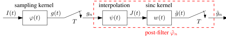
Fig. 17. Optimal post-filter applied to non-ideal low-pass samples (1-D case).
