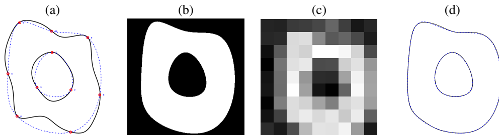
Fig. 11. The annihilable curve model is able to represent accurately non-annihilable curve (see, text in Section V-A3). (a) Consider a non-annihilable curve (dashed blue line) built using a cubic spline interpolation of a few samples (red circles) of an annihilable curve (solid black line). (b) Edge image associated with the non-annihilable curve. (c) Samples of the edge image ( 9 \times 9 pixels). (d) The reconstructed annihilable curve (solid black line) based on the samples in (c) is barely distinguishable from the ground truth non-annihilable curve (dashed blue line).
