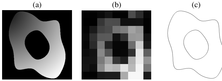
Fig. 9. Exact reconstruction of the annihilable curve C with minimum number of samples of the associated edge image I_C (see, Theorem 2). The discontinuity across the curve is f_0 = x + jy . (a) Modulus of the continuous domain edge image. (b) Modulus of the noiseless samples of the edge image (size: 9 \times 9 ). (c) Perfectly reconstructed annihilable curve C .
