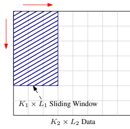
Fig. 4. The total number of shifts we can have when sliding a K_1 \times L_1 window over K_2 \times L_2 data block is (K_2 - K_1 + 1)(L_2 - L_1 + 1) .
