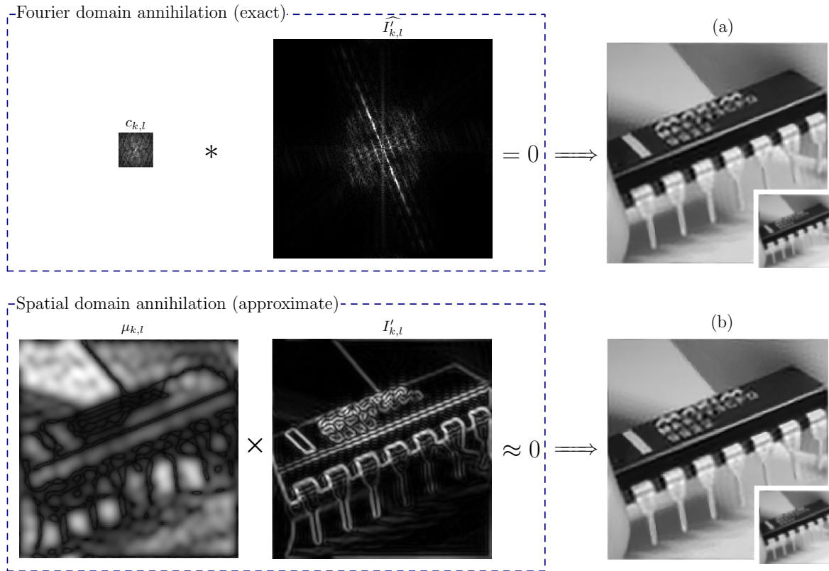
Fig. 8. Upsampling by a factor 3 of the small inset image in (a) and (b) using two methods: in (a) we use the exact Fourier domain formulation, in (b) we use the approximate spatial domain formulation. Either method yields a similar result: SNR between (a) and (b) is 34.44 dB (order of the FRI curve model: 31 \times 31 ).
