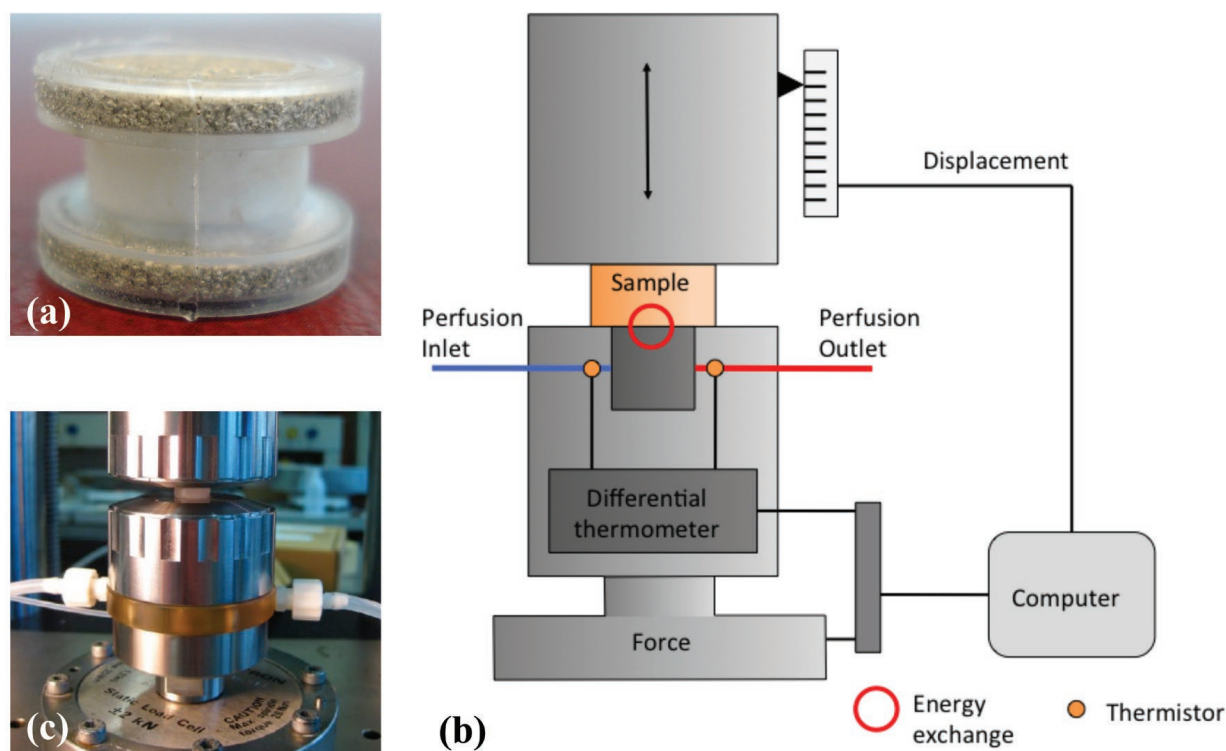
Fig. 1. (a) The encapsulation chamber made of a silicon membrane enclosing the cartilage sample between a steel filter and a non-porous rigid disc. (b) The principle of the calorimetric measurement is based on the differential temperature measurement of the inlet and outlet perfusion. The cartilage sample, placed in the encapsulation chamber, is clamped between two mechanical actuators mounted on a standard tension machine. (c) Picture of the deformation calorimeter.
