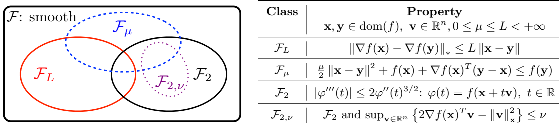
Figure 1: Common structural assumptions on the smooth function f .
