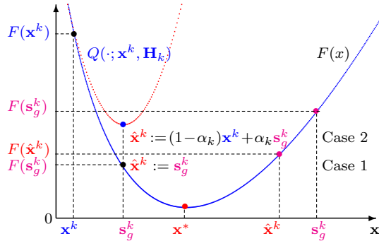
Figure 3: Illustration of the modified proximal-gradient method
