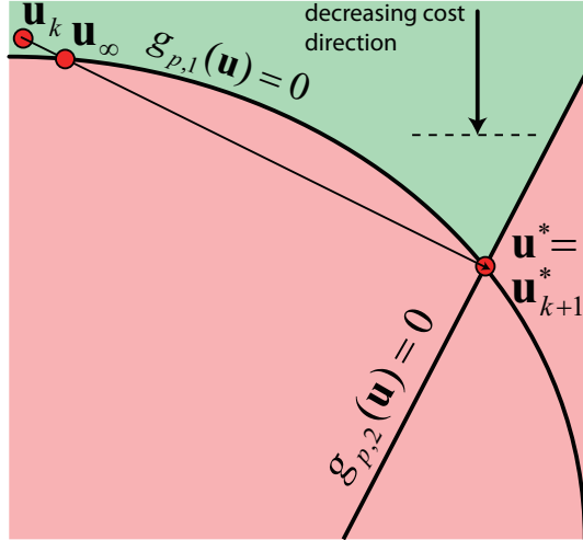
Figure 3: An example illustrating premature convergence, where one of the constraints becomes active and brings the filter gain to an arbitrarily small value. As the segment [\mathbf{u}_\infty, \mathbf{u}_{k+1}^*] is infeasible, the algorithm converges to \mathbf{u}_\infty without being able to proceed further.
