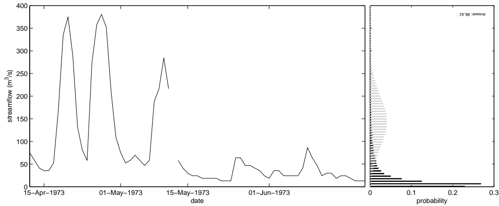
Fig. 2. The missing value in the flow time series can be guessed from the surrounding values (a guess would for example be the gray histogram). This will usually lead to a better guess than one purely based on the occurrence frequencies over the whole 40 yr data set (dark histogram) alone. The missing value therefore contains less information than when assumed independent.
