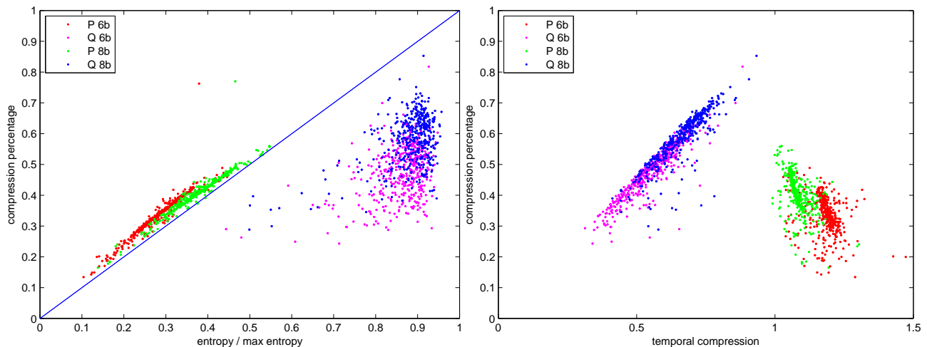
Fig. 7. Changes in results due to coarsening the quantization from 8 to 6 bits (8b and 6b) for precipitation ( P ) and streamflow ( Q ). For interpretation, we refer to the text.
