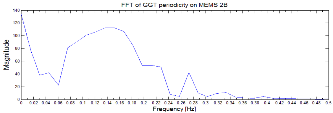
Figure 9. FFT of GGT periodicity; Peak at \sim 0.14 Hz
