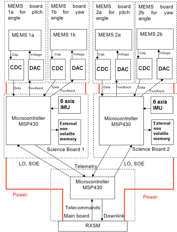
Figure 2. Diagram of GGES experiment setup
