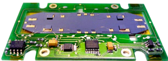
Figure 5. MEMS board showing the silicon micro-electro-mechanical sensor, and electronics to measure the displacement of the proof mass.
