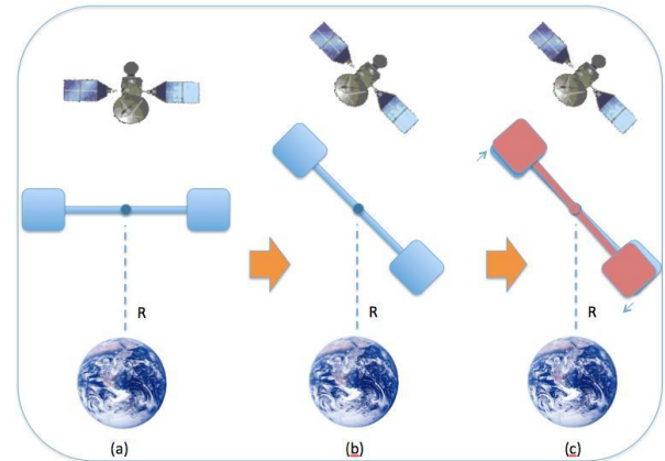
Figure 1. Diagram showing effect of the gravity gradient on an elongated proof mass. (a) the proof mass inside the satellite is perpendicular to the Earth. Both sides of the mass being the same distance from the Earth, there is no detectable effect. If the satellite rotates by a given amount (b), the mass inside also rotates. Since now one side is closer to the Earth and sees more gravity (c), the GGT will produce a displacement
