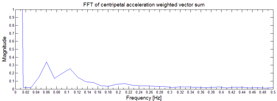
Figure 8. FFT of centripetal acceleration along REXUS roll axis during freefall; Peaks are observed at ~0.07 and ~0.11 Hz
