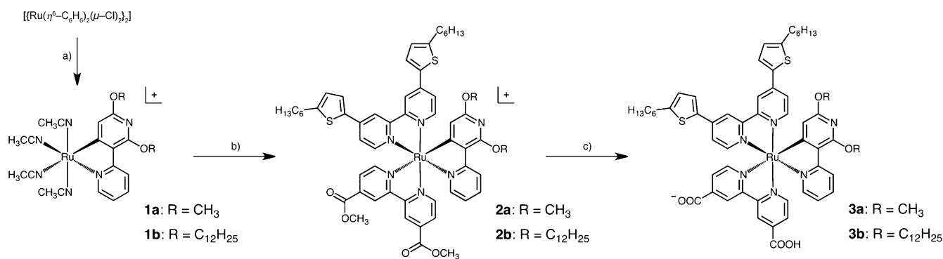
Scheme 1. Synthesis of complexes 3a and 3b . Charged complexes were isolated as PF 6 - salts. a) 2',6'-dimethoxy-2,3'-bipyridine or 2',6'-bis(dodecyloxy)-2,3'-bipyridine, NaOH, KPF 6 in MeCN ( 1a : 56%, 1b : 43%); b) 2,2'-bis(5-hexylthiophen-2-yl)-2,2'-bipyridine, 4,4'-dimethylester-2,2'-bipyridine in EtOH ( 2a : 48%; 2b : 45%); c) DMF, H 2 O, Et 3 N (3:1:1) ( 3a : 77%; 3b : 95%).
