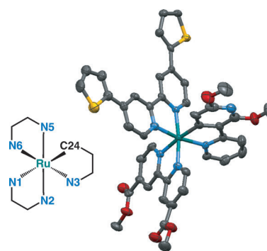
Figure 1. Crystal structure of 2a ·2CH 2 Cl 2 . Thermal ellipsoids are drawn at the 50% probability level. The counter ion, hexyl chains, hydrogen atoms, and solvent molecules are omitted for clarity. Additional information can be found in Table S1. N blue, O red, S yellow, Ru turquoise.
