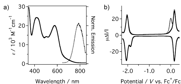
Figure 2. a) Steady-state absorption (—) and normalized emission spectra (---, λ exc = 580 nm), and b) differential pulse voltammogram (—) with a ferrocene internal standard (---) in dichloromethane of 3b . Scan rate of 100 mV s -1 with 10 mV pulses.
