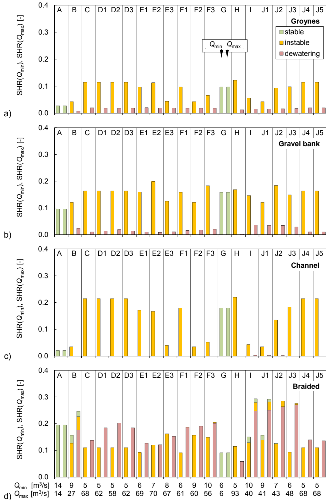
Figure 6.8: Suitability Habitat Ratio (SHR) for spawning brown trout for the off-peak Q_{\min} and the peak Q_{\max} discharge of the measured and simulated November conditions (Table 6.2), computed for the groynes (a), gravel bars (b), channel (c) and braided (d) reaches. The percentage of stable (green), instable (yellow) and dewatering (red) habitat is given for discharge changes from Q_{\min} to Q_{\max} and Q_{\max} to Q_{\min} , respectively.
