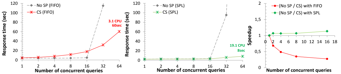
Figure 6: Evaluating multiple identical TPC-H Q1 queries (a) with a push-only model during SP (FIFO), and (b) with a pull-based model during SP (SPL). In (c), we show the corresponding speedups of the two methods of SP, over not sharing, for low concurrency.
