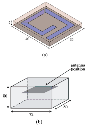
Figure 1. Simplified spiral antenna (a) and body model (b)
