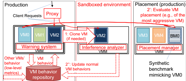
Figure 2: DeepDive overview, showing how it detects and mitigates the effect of interference on VM2.
