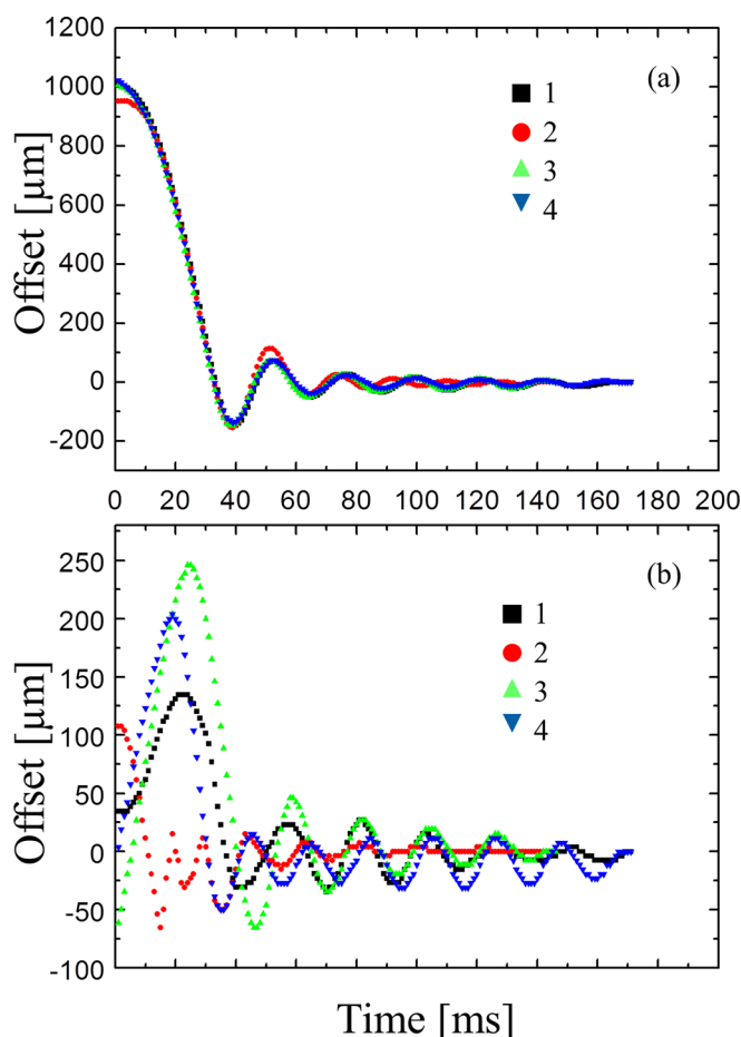
FIG. 6. Self-alignment trajectory of a foil (0.80 mg/mm 2 ) die as recorded by high-speed camera along (a) principal and (b) secondary axis. The die was repeatedly released at various initial offsets along the secondary axis, while initial offsets along main axis were kept the same within loading precision of the micropositioner.
