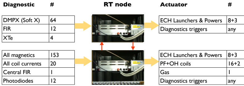
Fig. 1. Schematic representation of control system nodes and connections used for the experiments presented in this paper. Each nodes can run at a different clock rates and communicate with other nodes via a shared memory. Adapted from [5].
