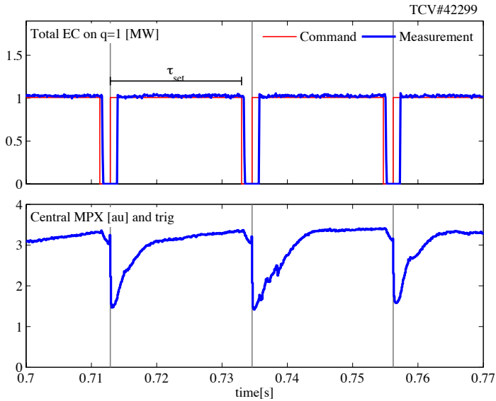
Fig. 3. Demonstration of sawtooth pacing in TCV. The gyrotron power is switched on after each detected crash and switched off after a pre-determined period \tau_{set} . The sawtooth crash is seen to appear shortly thereafter. The EC system hardware causes a short delay between the power command and obtained forward power. From [5].
