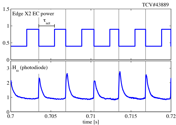
Fig. 4. Detail of ELM pacing: the EC power is switched off after the detection of each ELM crash. The power is switched back ON after a prescribed time, stimulating the appearance of the next ELM. From [5].
