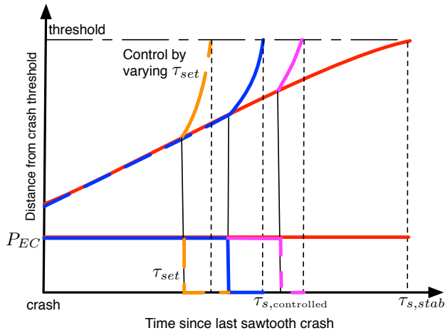
Fig. 2. Cartoon illustration of sawtooth pacing principle: the EC power which otherwise slows the evolution of the plasma towards the crash threshold is switched off during the sawtooth cycle, giving precise control of the sawtooth period by varying the switch-off time \tau_{set} (Figure from [5])
