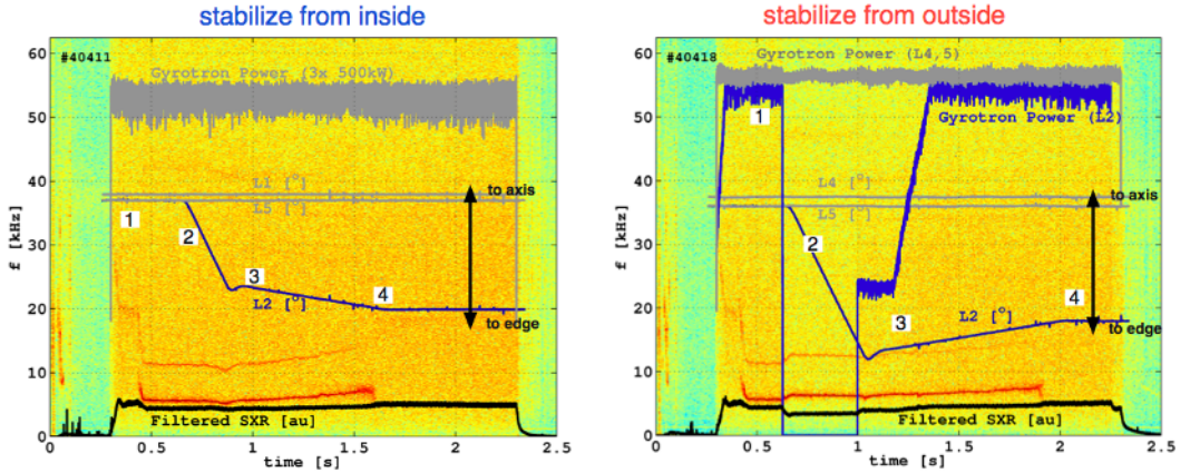
Fig. 5. Stabilization of NTMs by sweeping the ECCD deposition location towards the island from both inside (left) and outside (right). An NTM is first created by three gyrotrons (total 1.5MW) injecting co-ECCD at approximately \rho_\psi = 0.3 (1). Some time after the magnetic island is detected, one of the launchers is moved towards the location of the island (2) and then slowly scanned towards the expected location (3). When the mode disappears, the angle is held constant (4). Note that when stabilizing from the outside (right panel) the gyrotron power is temporarily switched off to allow the launcher angle to go to the requested location without depositing power on the island. From [5].
