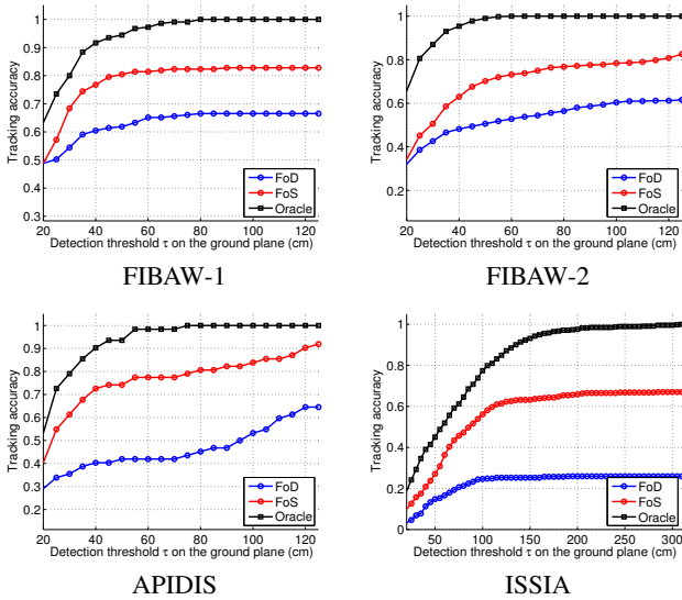
Fig. 5. Comparison of FoD and FoS tracking. The performance of FoS approaches that of the oracle and is decisively better than FoD, particularly in the accuracy range of \leq 100 cm. The results are obtained by fixing n = 1 . From left to right: results on FIBAW-1, FIBAW-2, APIDIS and ISSIA dataset.
