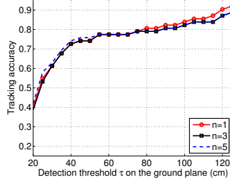
Fig. 7. Tracking performance with different settings of n , i.e. the number of BOM peaks used for training the unary potential.
