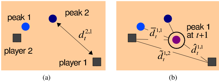
Fig. 4. Given the locations of the players and BOM at time t and t + 1 , we define a set of geometric primitives. These primitives will then be used to derive the features for learning \psi_1 and \psi_2 . (a) We define d_t^{j,k} as the distance between peak j and player k at time t . (b) We define \tilde{d}_t^{k,k'} as the distance between player k and player k' at time t , \hat{d}_t^{j,k} as the distance between peak j at time t + 1 and player k at time t , and \bar{d}_t^{j,j'} as the distance between peak j at time t and peak j' at time t + 1 .
