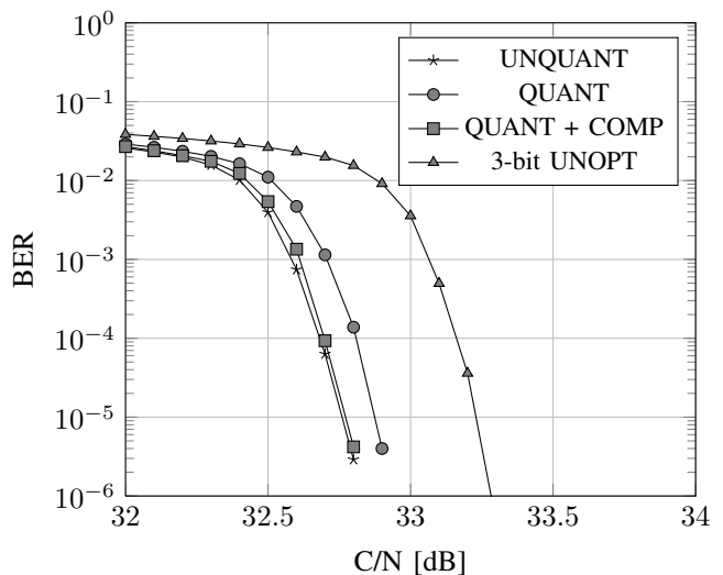
Fig. 11. BER vs C/N. UNQUANT: unquantized QAM; QUANT: system with quantized LLR; QUANT + COM: system with quantized and compressed LLR; UNOPT: unoptimized quantization; All the quantized system use a total of \bar{N} = 36 bits.
