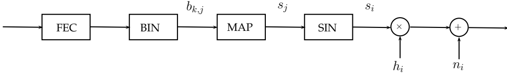
Fig. 1. Transmitter and channel models. FEC: Forward Error Correction; BIN: Bit Interleaver; MAP: Mapper; SIN: Symbol Interleaver.
