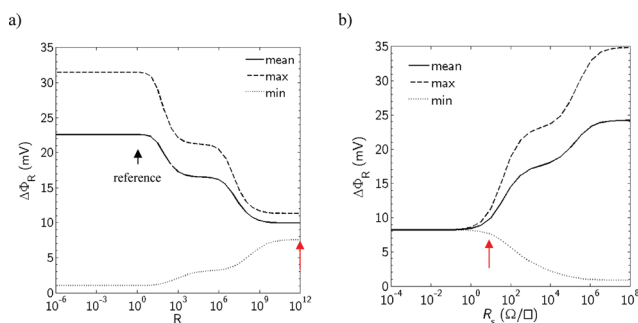
Fig. 6 Average, minimal and maximal potential drop in the solution for varying scale factor, R , i.e. reactions' exchange current densities, at R_s = 10 \Omega \square^{-1} (a), and for varying TCO sheet resistance, R_s , at R = 10^{12} (b), both for Design A, t_{sep} = 10 \mu m, h_e = 1 mm, and l_{el} = 5 mm. The black arrow in panel (a) depicts the reference case for the state-of-the-art catalysts and TCO resistance. The red arrows show the same R - R_s -conditions for the two different figures.
