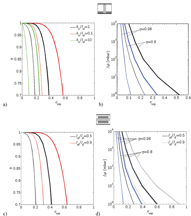
Fig. 12 (a and c) Current efficiency at \Delta p = 10 mbar as a function of separator porosity at t_{\text{sep}} = 10 \mu\text{m} (thin lines) and t_{\text{sep}} = 500 \mu\text{m} (thick lines) for various component dimensions in Design A (a), and for h_e = 1 \text{ mm} and l_{\text{el}} = 1 \text{ mm} in Design B (c). (b and d) Differential pressure at \eta = 0.8 (black) and 0.98 (blue) as a function of separator porosity at t_{\text{sep}} = 10 \mu\text{m} (thin lines) and t_{\text{sep}} = 500 \mu\text{m} (thick lines) for h_e = 1 \text{ mm} and l_{\text{el}} = 1 \text{ mm} in Design A (b), and Design B (d), where l_{\text{el}}/l_d = 0.5 (solid lines) and l_{\text{el}}/l_d = 0.9 (dotted lines).
