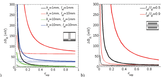
Fig. 13 Average ohmic potential drop, \Delta\Phi_{\text{R}} (solid line), and average ohmic potential drop minus the average potential drop over the separator, \Delta\Phi_{\text{R}} - \Delta\Phi_{\text{R,sep}} (dotted line), as a function of separator porosity for t_{\text{sep}} = 10 \mu\text{m} (thin lines) and t_{\text{sep}} = 500 \mu\text{m} (thick lines), for various dimensions of Design A (a) and Design B at h_e = 1 \text{ mm} and l_{\text{el}} = 1 \text{ mm} (b).
