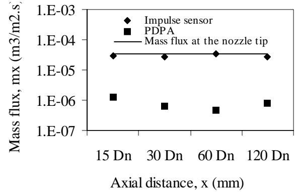
Figure 8. Mass flux variation with axial distance from the tip of the nozzle. Here, Dn indicates diameter of the of the nozzle tip of 3.10 mm.
