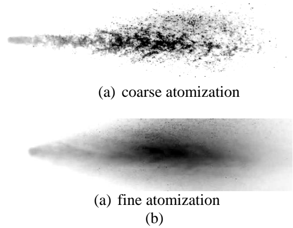
Figure 4. Spray images.
