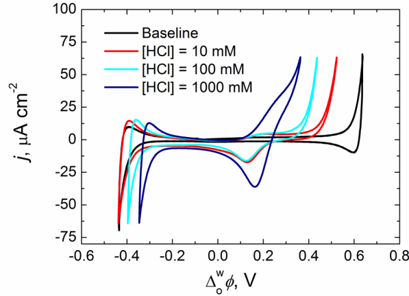
Figure S2. pH dependence of the voltammograms of 5 mM FcMeOH in DCB. Baseline: 5 mM BATB in DCB and 10 mM HCl.
