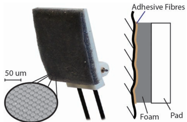
Fig. 1. From left to right: SEM micrograph of the fibre adhesives, adhesive pad with micro-fibres and a layer of foam, and a schematic representation of how the foam increases the compliance of the pad and distributes the peel off force.
