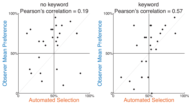
Figure 6. Plotted are the results of the automated selection versus the psychophysical (observer mean preference) results, both without the keywords and also with the keywords. The keywords, for most images, improved the results by moving the points closer to the diagonal line, which is the ideal.
