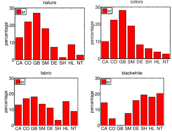
Figure 2. Semantic relatedness values sr for four keywords as indicated in the titles for the eight quality attributes. The keywords colors and nature both imply the importance of Colorfulness (CO) and Gamut Boundary (GB), whereas fabric and blackwhite relate stronger to Neutrals (NT) and Details (DE). Note that colors and nature are similar in terms of their meanings for ICC rendering intents.
