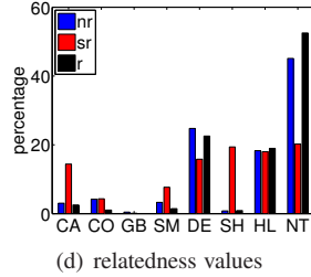
Figure 3. Same images as in Figure 1, but with a semantic context indicated by the keyword in the caption. The bar graphs show the numeric nr_q(j) , semantic sr_q(w) and united relatednesses r_q(j,w) , respectively. Top: the semantic context colors reduces the relatedness to Details (DE) and increases it for Color (CO) and Gamut Boundary (GB). Bottom: the semantic context blackwhite makes Details (DE), Highlights (HL) and Neutrals (NT) the dominant quality attributes.
