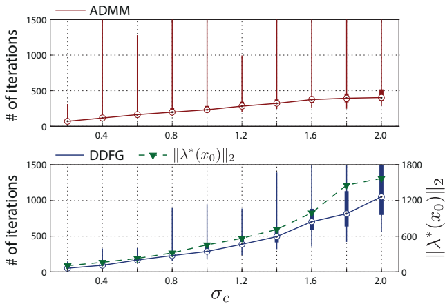
Fig. 1: Number of iterations to convergence under ADMM and DDFG for a network of 10 coupled double-integrators with \sigma_s^i = 1 and \sigma_c^i \in \{0.2, 0.4, \dots, 2.0\} . The median of \|\lambda^*(x_0)\|_2 is depicted in the lower plot.
