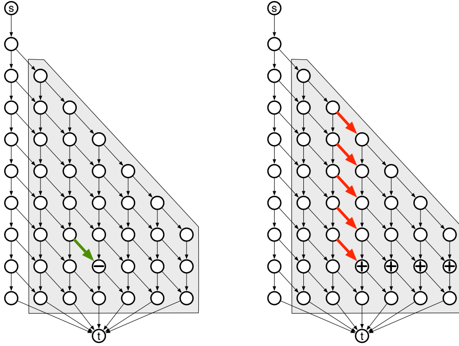
FIGURE 5. Coefficient vectors of inequalities (5) (left) and (6) (right).
