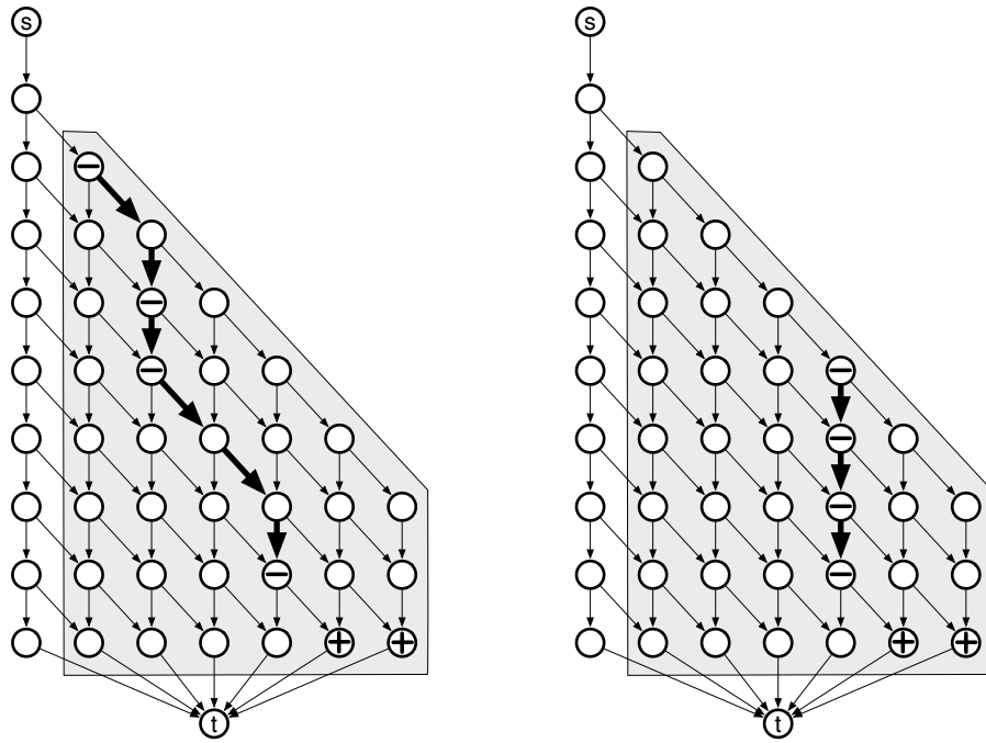
FIGURE 3. Coefficient vectors of two SCIs with the same bar \bar{\text{bar}}_{8,5} .
