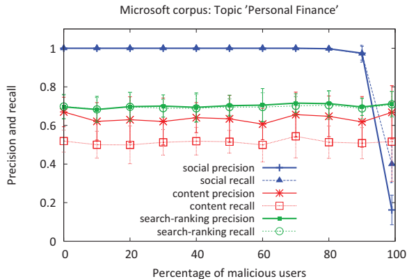
Figure 10: Microsoft corpus: Performance of different components for the category “finance”. The search-ranking component has higher precision and recall than the content component.
