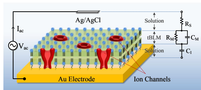
Figure 1. Schematic view and equivalent model of a two-electrode electrochemical cell with an Ag/AgCl counter electrode and a gold working electrode coated with a tBLM. The impedance of the large ( >1 cm 2 effective area) counter electrode is negligible when the electrolyte solution comprises enough chloride ions (usually \geq 0.1 M).
