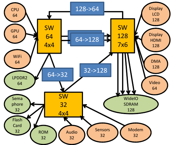
Figure 11: Topology
