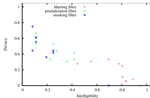
Fig. 1: Intelligibility vs. privacy for different filters.
