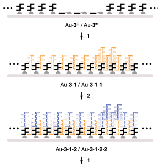
Figure 15. Possible mechanisms of mixed zipper architectures integrating overzipped domains.
