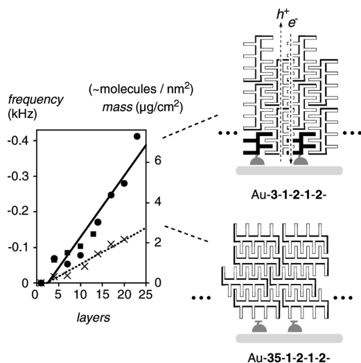
Figure 16. QCM frequencies (with linear curve fit) as a function of the number of theoretical layers of zipper assembly Au-3-(1-2) n (●, ■) and LBL assembly Au-35-(1-2) n (X).
