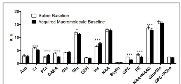
Fig. 3: Metabolite concentration (mean \pm s.e.m., n=3 ) of ^1\text{H} spectrum using the spline baseline (blue) or the in vivo measured macromolecule baseline (* p<0.05 , *** p<0.001 ).
