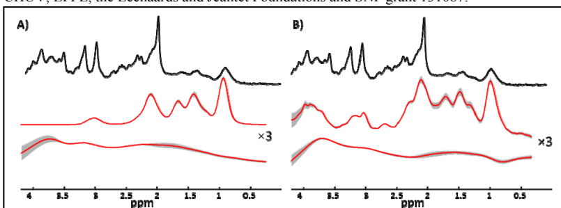
Fig. 2.A) ^1\text{H} NMR spectra (top, n=64 ) with the built-in LC Model spline baseline (A).
