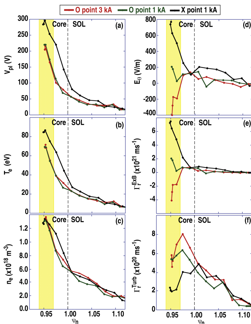
Fig. 2. Data from the midplane scanning probe showing profiles of: (a) Plasma potential, (b) electron temperature, (c) electron density, (d) poloidal electric field, (e) ExB flux from the previous field and (f) turbulent radial particle transport from fluctuations. The profiles are plotted vs poloidal normalized flux. The expected island location, as TRIP3D modeling is shown as a shaded box and the position of the LCFS is indicated by a vertical dashed line.
