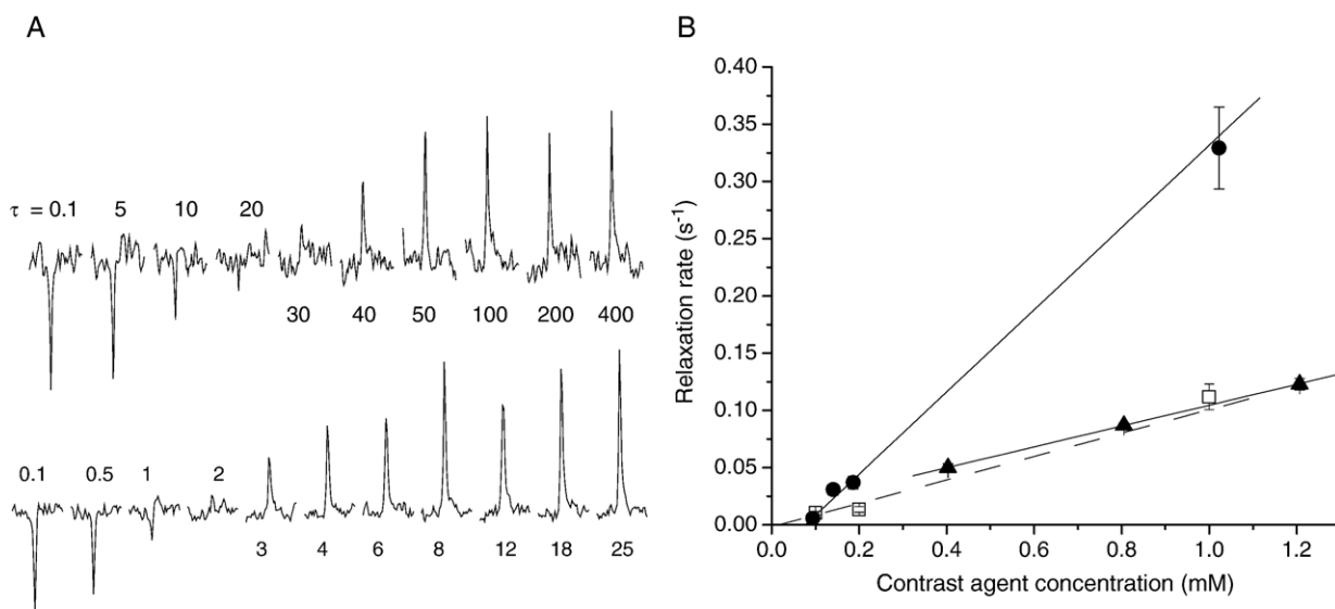
Fig. 3. The effect of contrast agents on lithium-6 transverse relaxation times. (A) Series of inversion recovery spectra for a LiCl solution in H 2 O with 0.05 mM (upper panel) and 1 mM (lower panel) of Omniscan. Inversion times are mentioned for each individual spectrum. (B) Determination of the relaxivity for the Magnevist in H 2 O (●), Omniscan in H 2 O (▲) and Omniscan in D 2 O (□) solutions. Error bars represent standard deviations of the inversion recovery curve fits.
