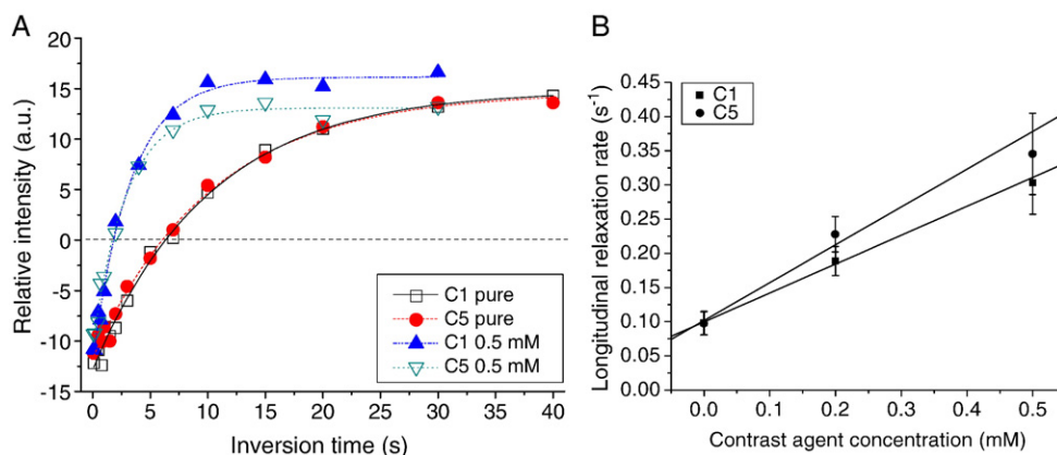
Fig. 2. Effect of Omniscan on the glutamate carboxyl carbon T_1 . (A) Inversion recovery curves of the glutamate carboxyl carbons at different concentrations of Omniscan. (B) A linear fit of the relaxation rate R_1 ( s^{-1} ) versus the concentration of Omniscan (mM) to determine the relaxivity of the carbons of the carboxyl groups of glutamate. Error bars represent the standard deviation on the inversion recovery fit.
