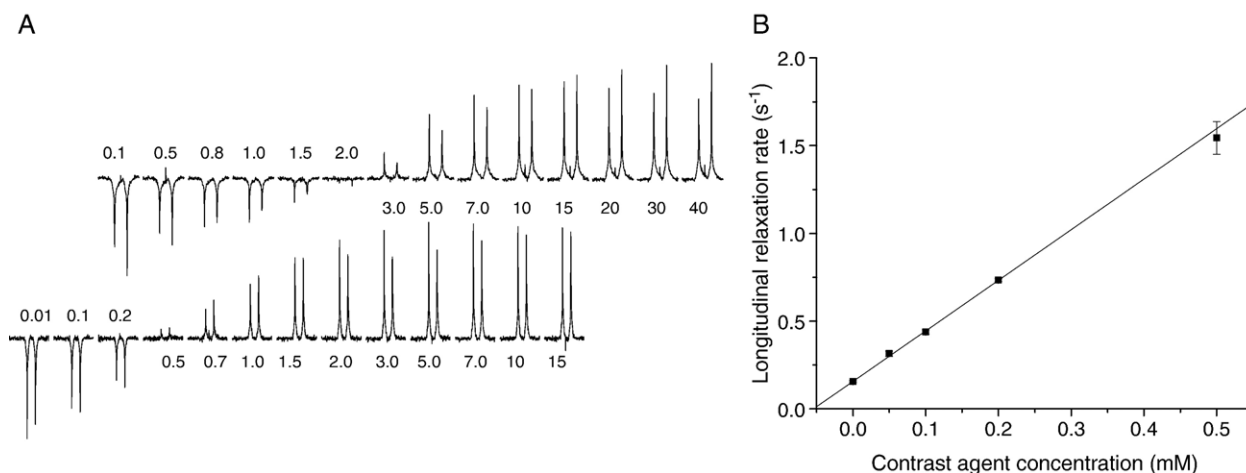
Fig. 1. Effect of Omniscan on formic acid ^{13}\text{C} T_1 . (A) Series of ^{13}\text{C} spectra of formic acid in the presence of 0.05 mM (upper panel) and 0.5 mM (lower panel) of the contrast agent Omniscan. The signal is a doublet since no decoupling was used. Inversion times \delta (s) are indicated for each trace. The inversion null can be seen at 2.0 and 0.5 s, respectively. (B) Linear fit of the relaxation rate R_1 (s) versus the Omniscan concentration [CA] (mM) to determine the relaxivity. Error bars represent the standard deviation of the T_1 , and fits are too small to be visible for the lower concentrations.
