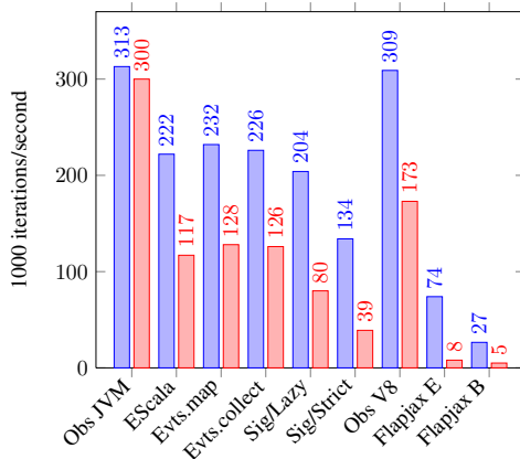
Figure 4: Propagation performance of a single event through a linear chain of 100 nodes (blue/left) or a fan with a fanout of 100 (red/right) in 1000 events propagated per second.
