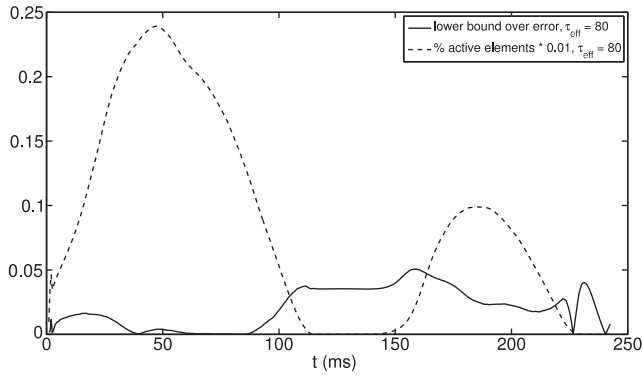
Fig. 3. Effectivity index \theta^{\text{low}} and percentage of active Bidomain elements for \tau_{\text{eff}} = 80 .
