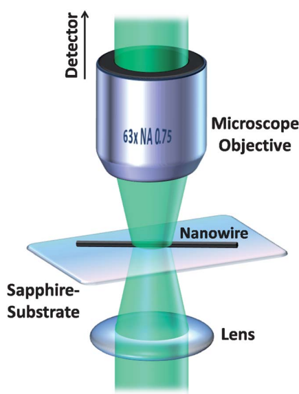
Fig. 1 A schematic drawing of the transmission Raman scattering from single nanowires.
