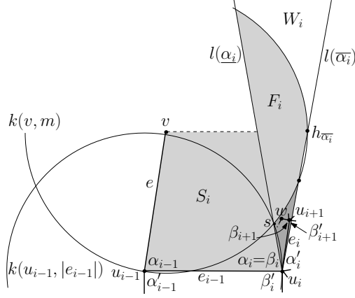
Figure 5: The setting for Lemmata 8–12. The dark-shaded region is R_i . To improve the readability, angles and edge lengths in the illustration do not correspond to actual angles and edge lengths.
