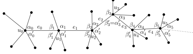
Figure 4: An embedding of C^* .
