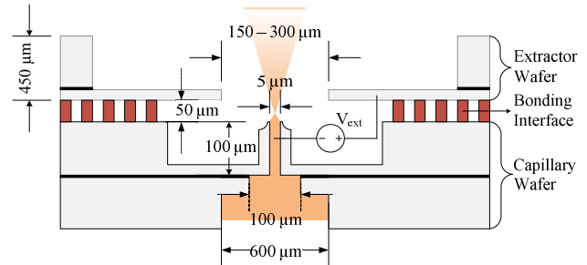
Figure 1: Cross-section view of the integrated thruster module depicting the thruster operation principle. The beam emission is induced by the large potential difference applied between the liquid and the extractor.
