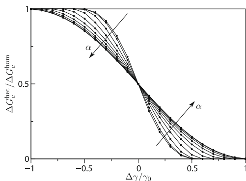
Figure 3. Nucleation Gibbs free energy barrier of a hexagonal crystal forming on an isotropic and flat substrate surface as a function of \Delta\gamma/\gamma_{st0} = (\gamma_{ef} - \gamma_{sf})/\gamma_{st0} for various orientations of the nucleus measured by the angle \alpha between the c -axis and the normal to the substrate surface. (From Mariaux [14].)
