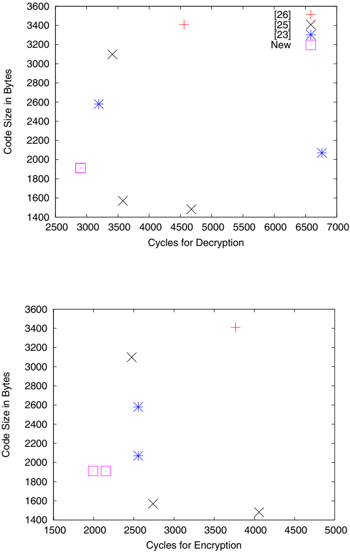
Fig. 2. Code size versus cycle count for decryption and encryption of different AES-128 AVR implementations
