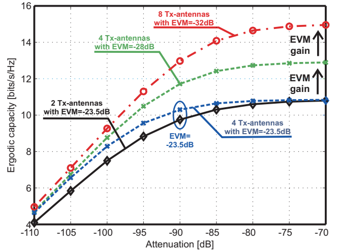
Fig. 2. Impact of increasing the number of Tx-antennas on ergodic MIMO channel capacity with two receive antennas under a constant power constraint.
