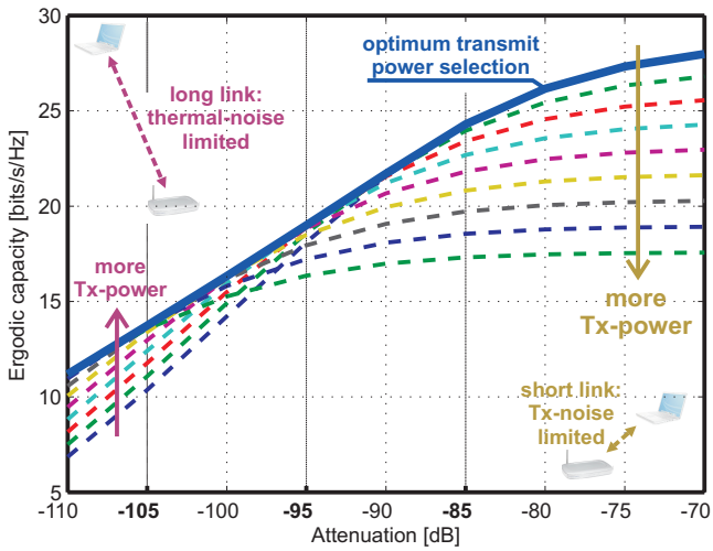
Fig. 3. Impact of increasing the Tx-power on ergodic capacity as a function of the channel attenuation in a 4 \times 4 MIMO system.
