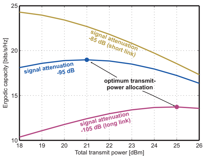
Fig. 4. Impact of increasing the Tx-power on ergodic capacity for -85 dB, -95 dB, and -105 dB attenuation in a 4 \times 4 MIMO system.
